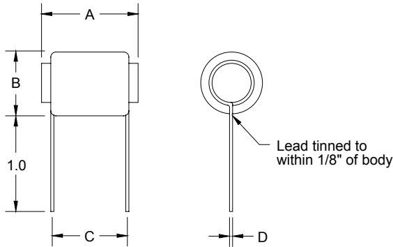
Dimensions: Inches
